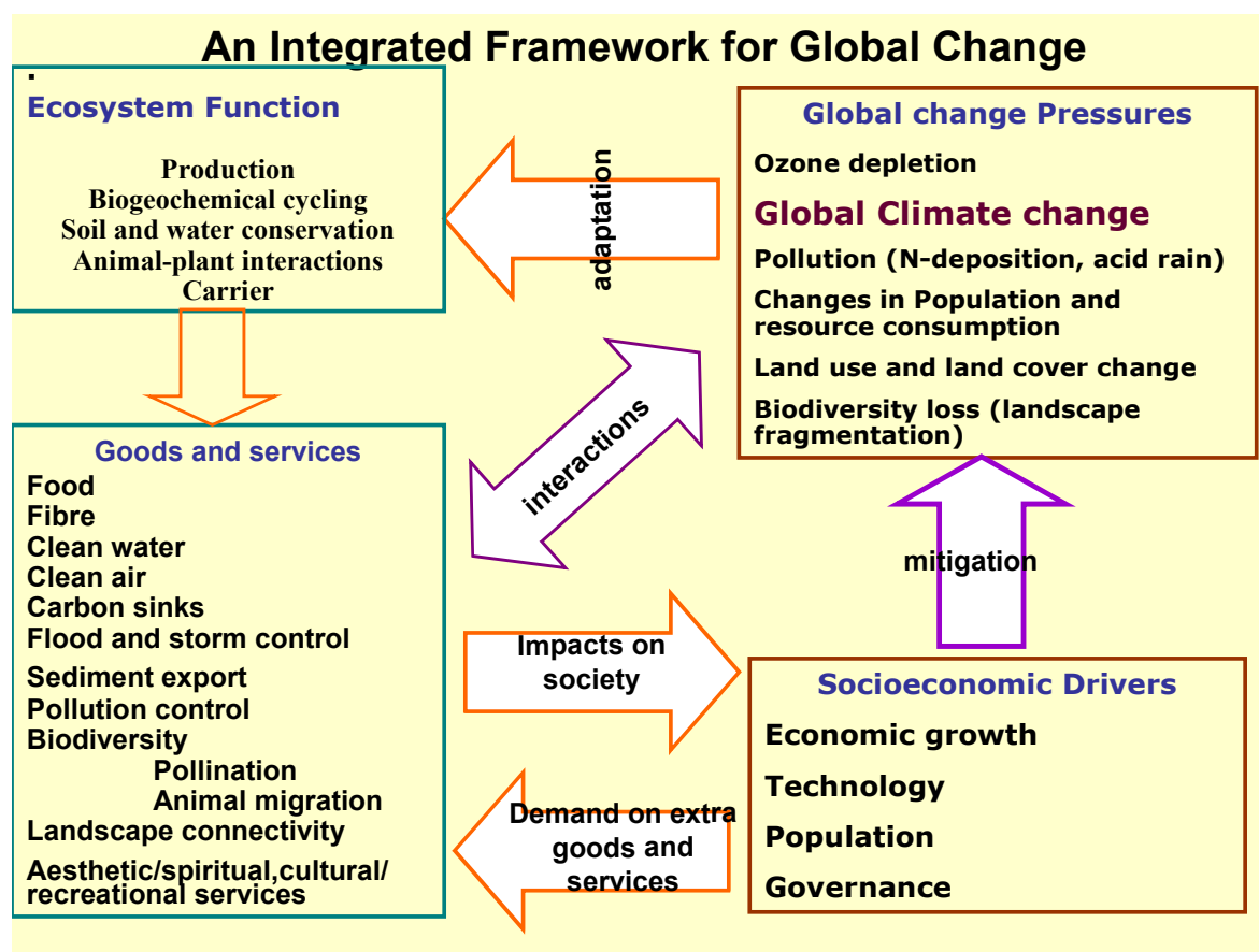
Figure 1: Climate change in the context of global change and the interaction between these changes, their drivers (socio-economic pathways), the ecosystem functions and the goods and services that ecosystems provide. Modified from IPCC (2001c) and Gitay et al (2001)
