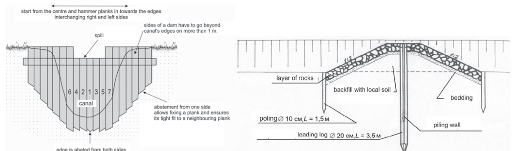
Figure 3 Overflow piling block made of planks (front view, left) and rock-filled block with piling wall (cross view, right) (From Kozulin et al. 2010).
